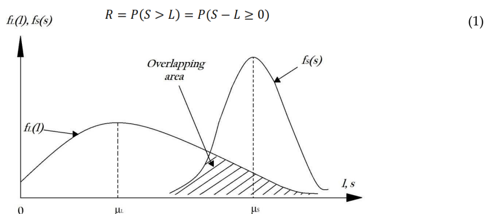
Figure 2. Probability density function for material structure load and strength [4].
